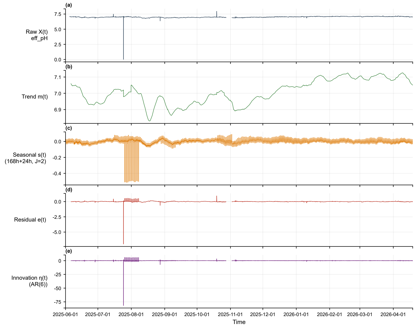
Multi-scale decomposition — eff_pH (effluent, hour) [2025-06-01~2026-04-19]
